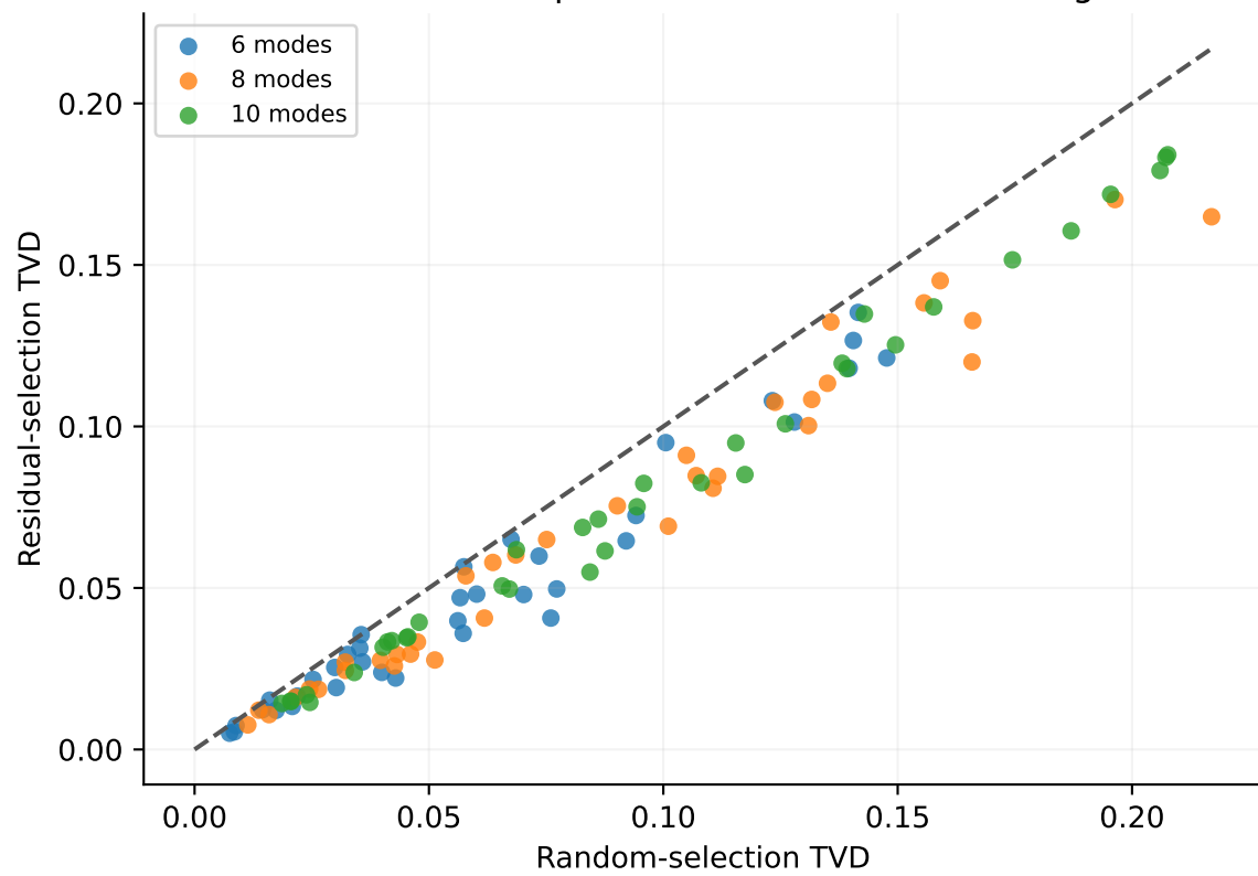
Same shortlist queries and fitted feature budget
